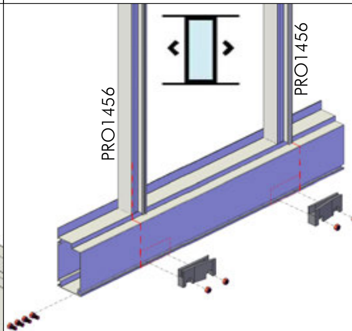
OPTION: SD (sliding door)
